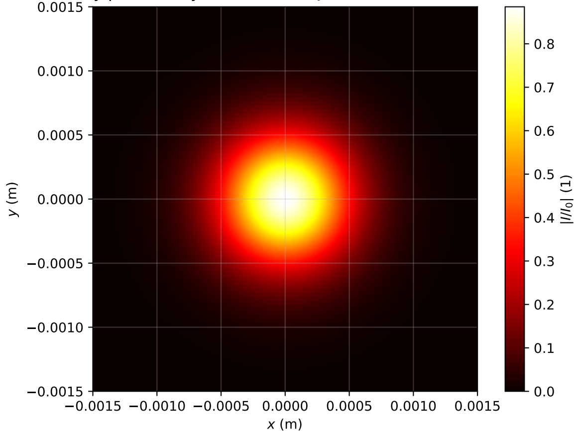
Intensity profile I(x, y, z = 1.194m)/I_0 , \text{Pin}=0.3\text{Pcr} , artificial time
